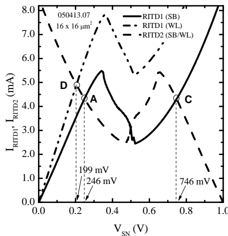
Fig. 4 Load line analysis during write to logic low (WL) cycle, from point C to D to A.
