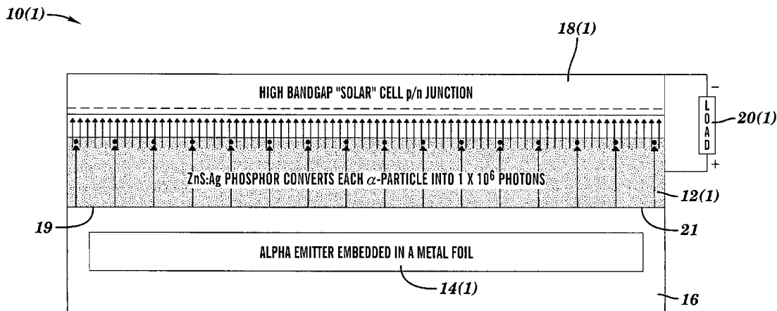
SCHEMATIC OF AN ALPHA VOLTAIC BATTERY
