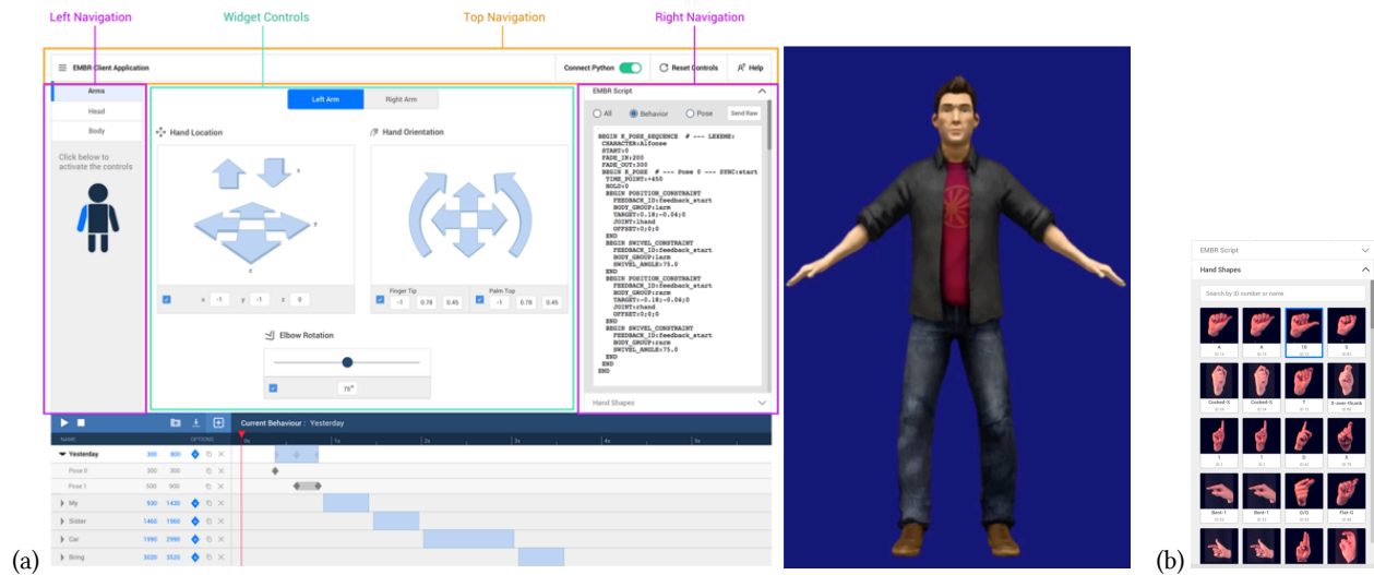
Figure 2: (a) Final version of user interface, (b) alternate view of Right Navigation with Hand Shapes section expanded.
