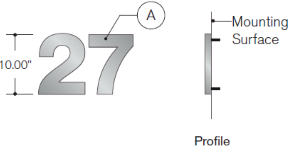
Dimensional Copy Painted, 1" Deep Custom Cast Aluminum Font: Neue Haas Grotesk Display 75 Bold Brushed - Vertical Grain
