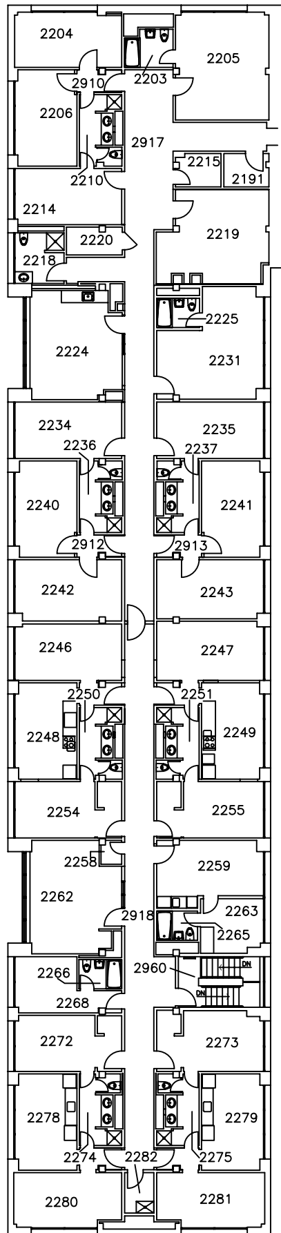
Bldg 050C NTID Residence Hall Second Floor Plan
