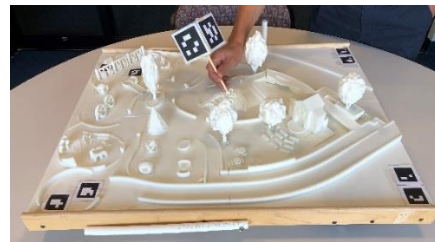
Fig. 1. 3D printed version of playground map, shown with user holding pointing stylus.
