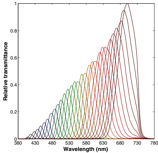
Fig. 1. Spectral transmittance factor of a wide-bandwidth CRI Varispec LCTF, circa 2000.
