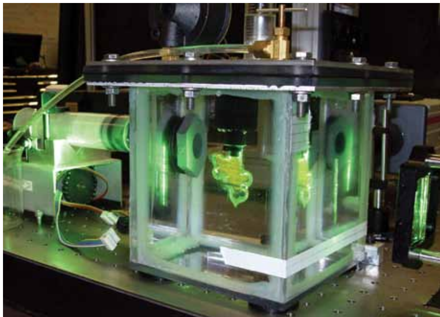
Particle Image Velocimetry: The alveolar sac model is housed in a glycerin-filled chamber and is connected to a computer-controlled syringe pump that draws a negative pressure on the fluid inside the chamber. The pressure is altered to expand and contract according to the applied motion of the pump, which mimics a realistic breathing curve.
