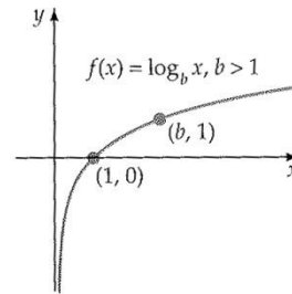
Logarithmic function
