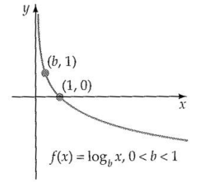
Logarithmic function
