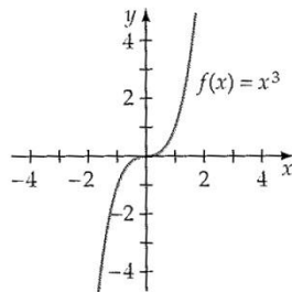
Cubing function
