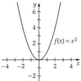
Squaring function
