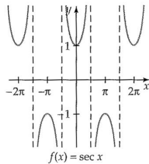
Secant function
