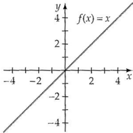
Identity function
