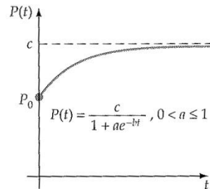
Logistic function
