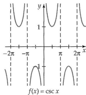
Cosecant function
