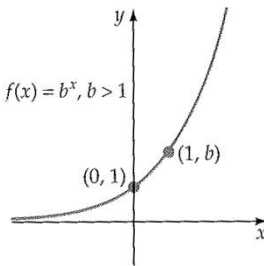
Exponential function
