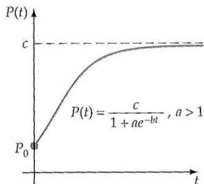
Logistic function
