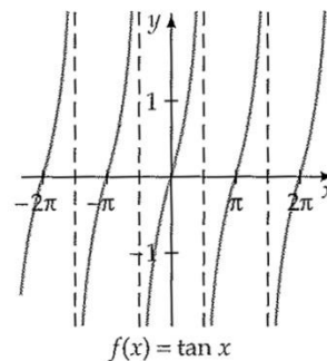
Tangent function
