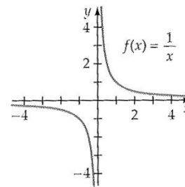
Reciprocal function
