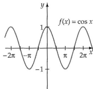
Cosine function
