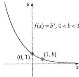
Exponential function
