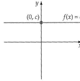
Constant function
