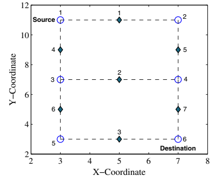
Fig. 7. Network topology for routing simulations. Hollow circles represent the legitimate nodes and diamonds represent potential eavesdropping locations.
